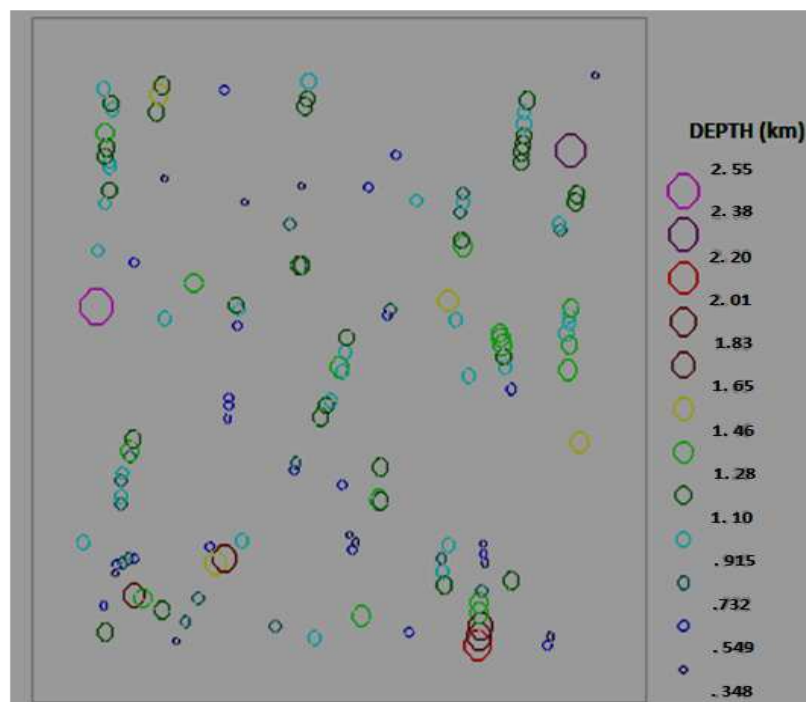
Fig.9: Depth and contact location from Analytic Signal Method (ASM).
